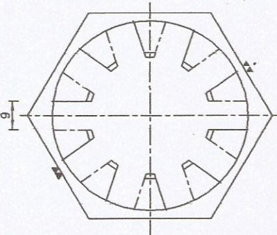
CASTLE NUT (PART NO.M42X1.5DIN937.6)
